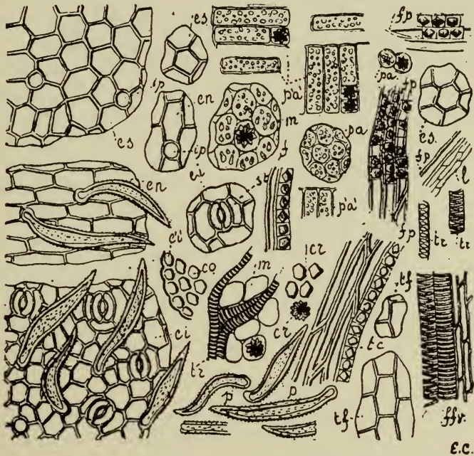
FIG. 61. — Powdered Senna. co , collenchymatous cells; cr , prismatic and cluster crystals; ei , ei' , lower epidermis; en , neural epidermis; es , upper epidermis; ffv , debris of fibrovascular bundles; f , fp , lignified fibres from midrib or veins; ip , scar of hair; l , bast; p , hair; pa , pa' , palisade cells; st , stomata; tc , cells with calcium oxalate; tf , cortical tissue of midrib; tr , vessels. \times 240 . (Greenish and Collin.)
